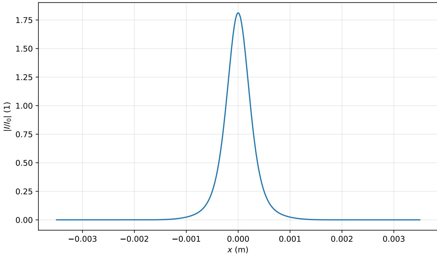
Intensity profile I(x, y = 0, z = 1.433m)/I_0 , P_{in}=1.0P_{cr} , artificial time
